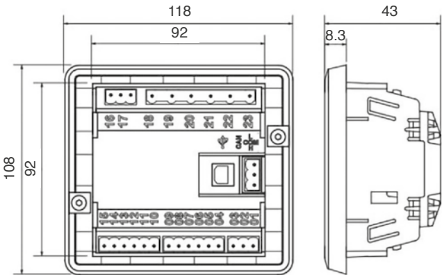
EOB-3000® Dimensions
