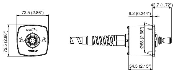
JLP/CH and JLP/B dimensions
