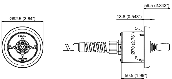
J/CH and J/B dimensions
