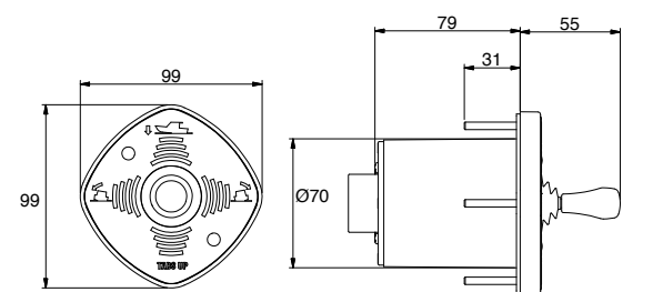
J/B-LED dimensions
