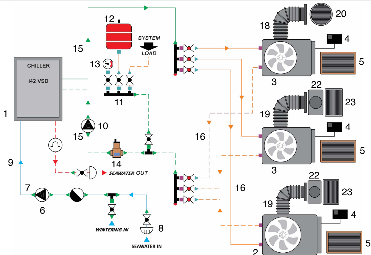
CHILLER i42 + 3 FANCOILS CONFIGURATION EXAMPLE
