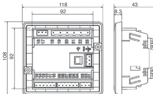
EOB-3000® dimensions
